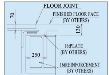
IRON FRAME SUPPORT BEAM
